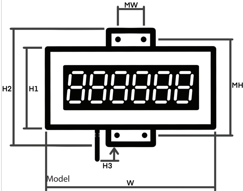
Front Profile
